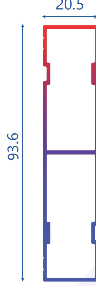
T.2353 0.968 KG/MT 3 KANALLI YAN KASA
